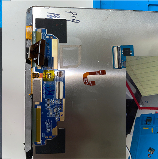
Samsung Tab A LCD and Board Replacement
